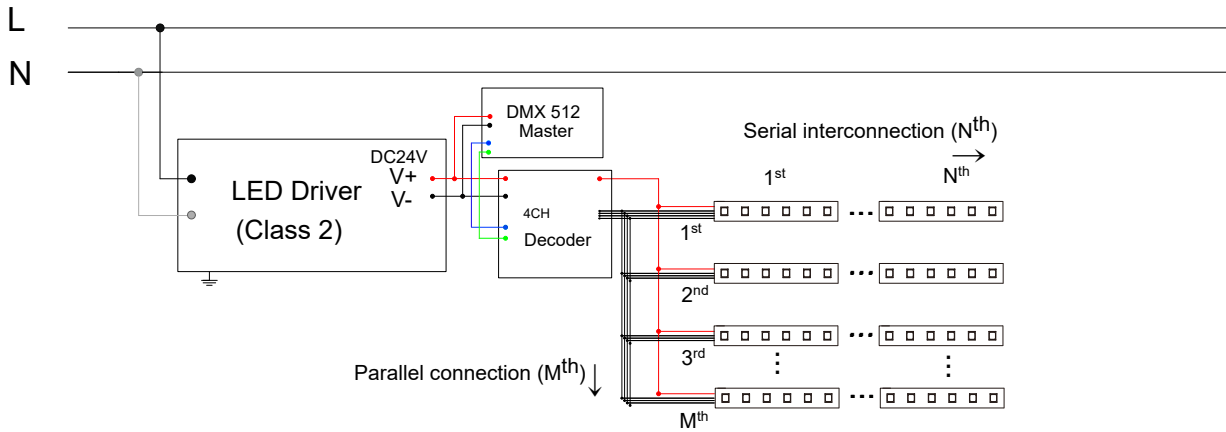
. LED Driver + NPB C5 ( DMX, RGBW )
